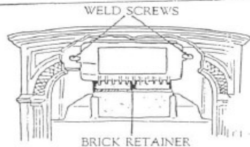
FIG. 4 POSITION OF UPPER FIREBACK
