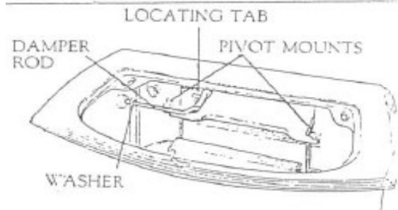
FIG. 3 POSITION OF DAMPER AND DAMPER ROD
