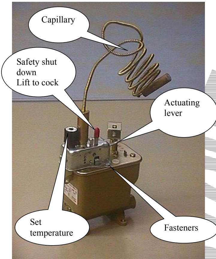
FIG 9 AQUASTAT FITTED
