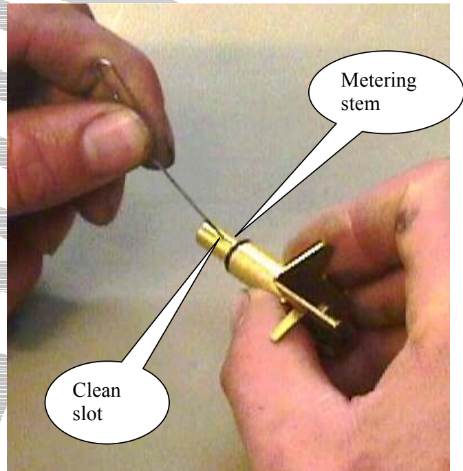
FIG 8 CLEAN METERING STEM
