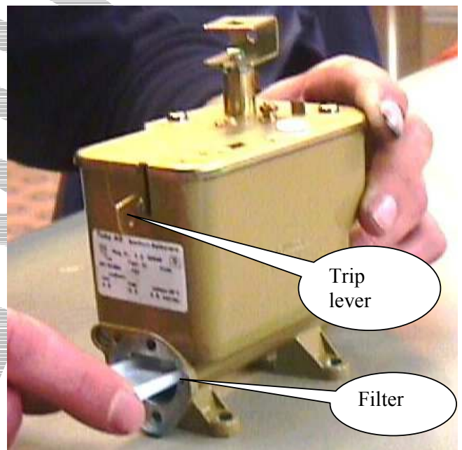
FIG 4 REMOVE FILTER
