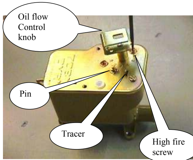
FIG 1 HIGH FIRE SCREW
