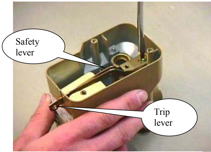
FIG 5 REMOVE FLOAT MECHANISM SCREW
