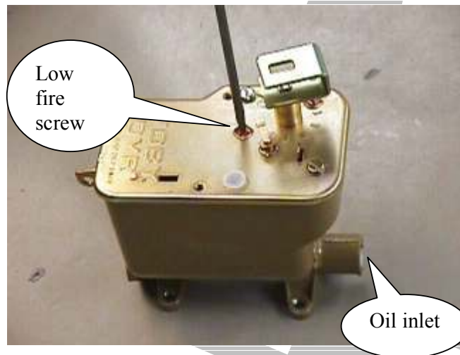
FIG 2 LOW FIRE SCREW
