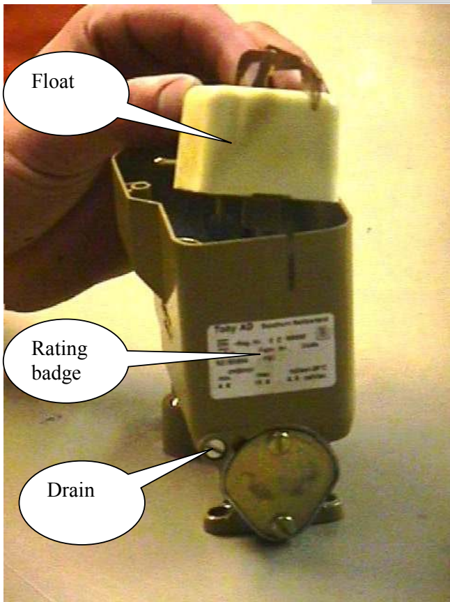
FIG 6 REMOVE FLOAT MECHANISM
