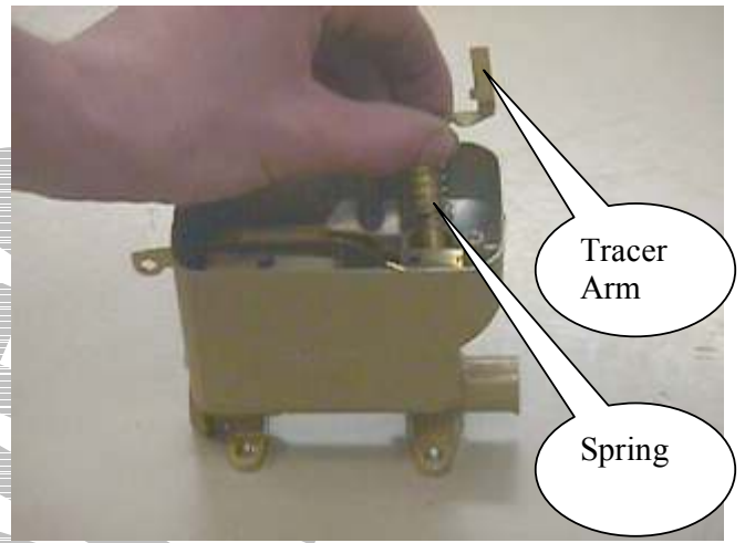
FIG 7 REMOVE METERING STEM
