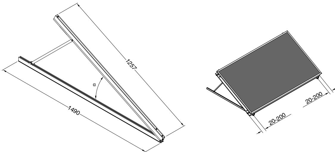
Figure 9 EURO TRIC F horizontal for 35° - 50°
