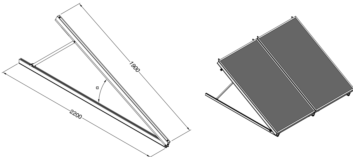
Figure 10 EURO TRIC F vertical for 37° - 50°
