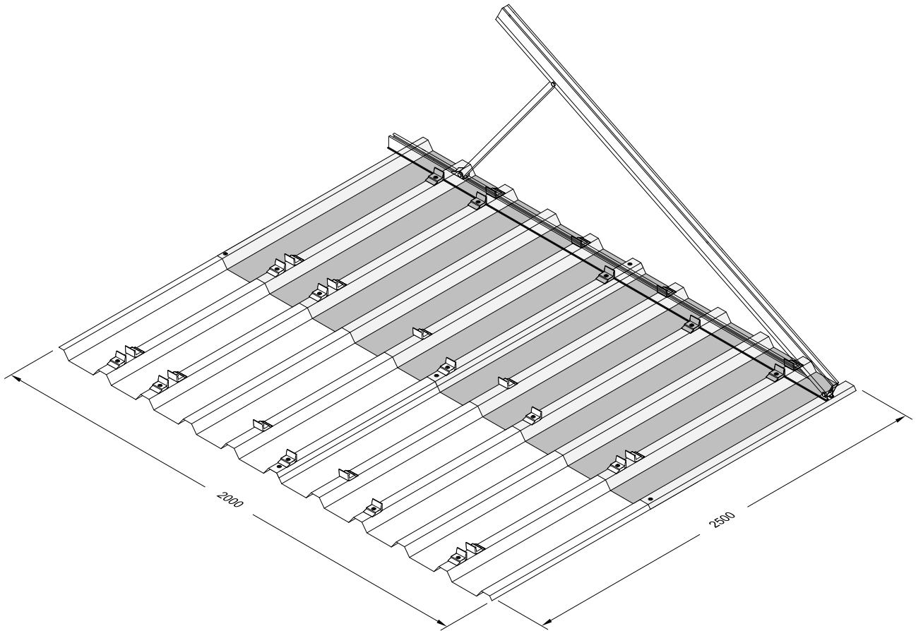
Figure 17 Gravel board basic and extension sets for vertical installation (prod. no. 192 020 76)
