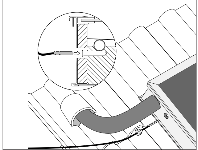
Figure 25 Pull sensor through rubber plug and insert sensor tip into sensor sleeve. Screw in rubber plug again.
