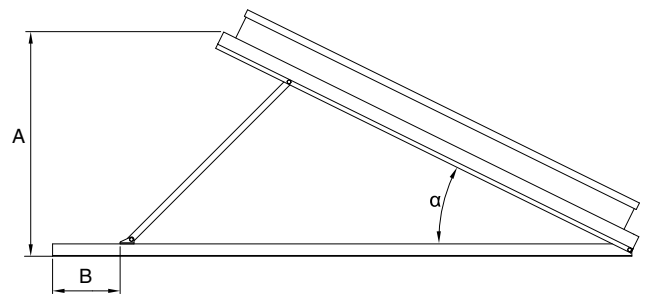
Figure 12 Collector inclination and setup dimensions
