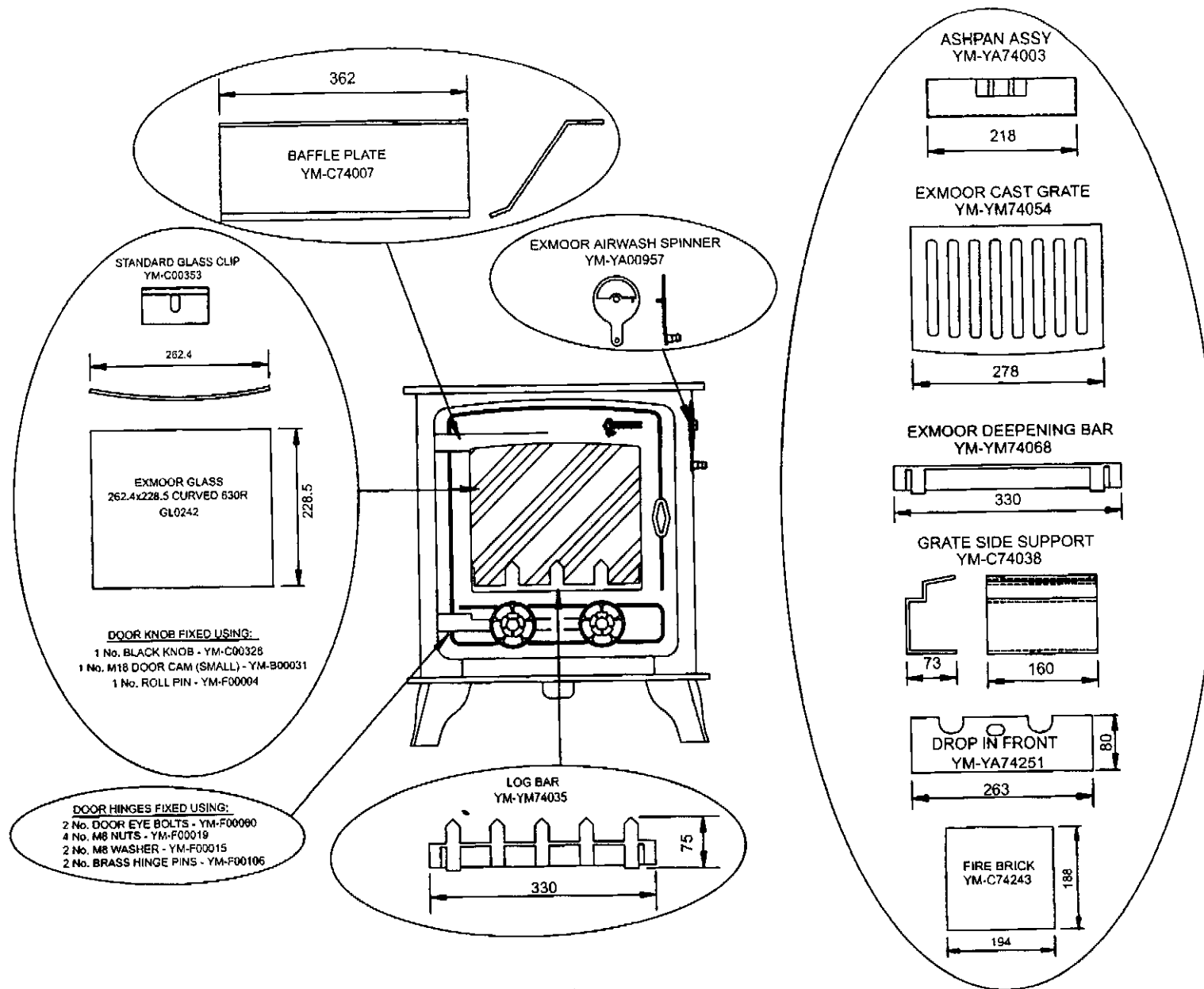
EXMOOR WOOD STOVE
