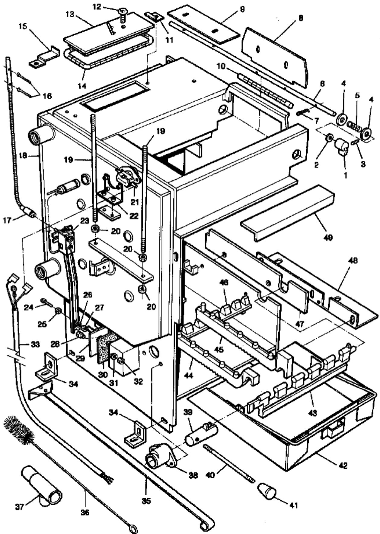
RAYBURN 355SFW/345W - BOILER, DAMPERS, THERMOSTATS, GRATE & RIDDLING ASSEMBLY
