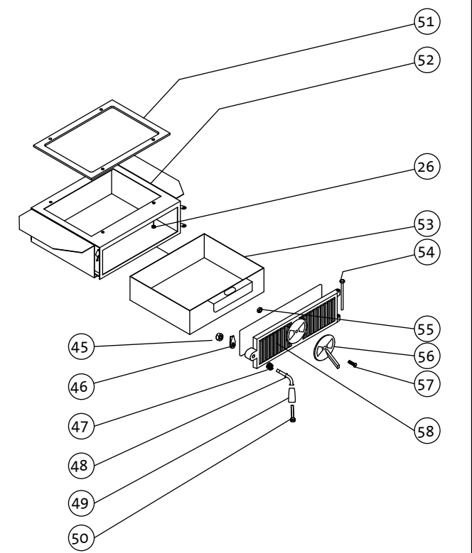
Exploded view/Deleliste F 3 MF Jøtul AS Fredrikstad, Norway Draw.no: 3-2944-P00 Date: Mars 05
