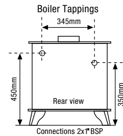
Approx. Weight: 94 - 100Kg
