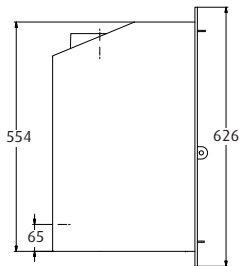
WESTFIRE.UNIQ.35 / INSERT 4-SIDED FRAME WEIGHT: 75 KG
