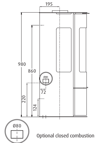
WESTFIRE.UNIQ.36 WESTFIRE.UNIQ.37 WEIGHT: 90 KG
