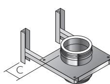
Cantilever Support Adjustment
