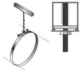
Ceiling Hanger
